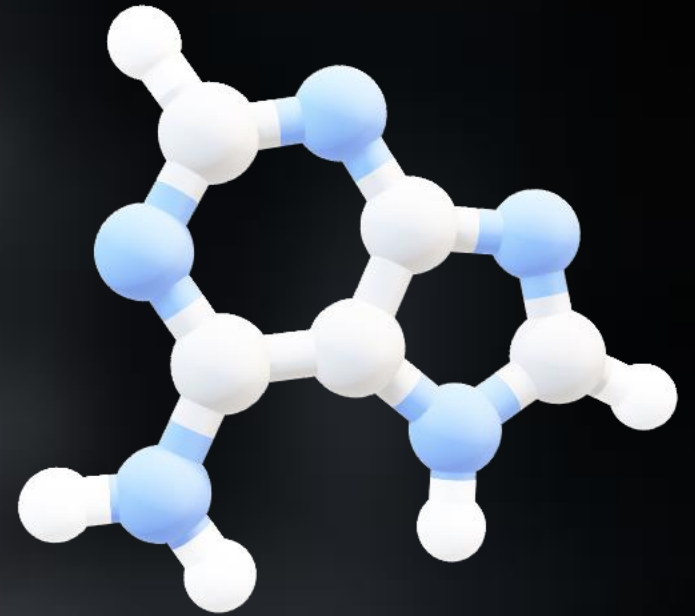
Nitrogen base
