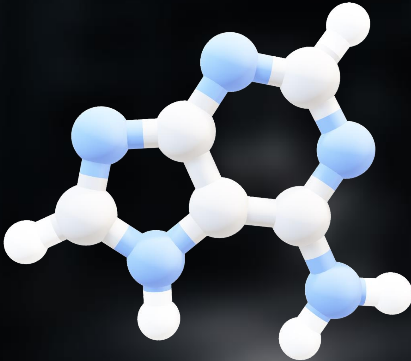
Adenine
