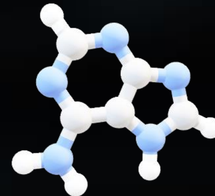
Nitrogen base
