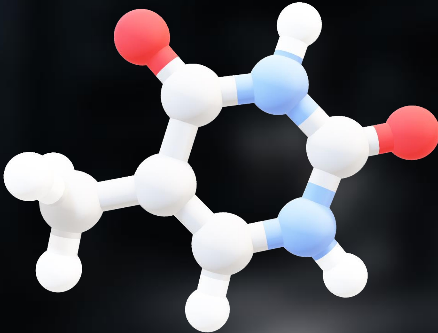
Thymine
