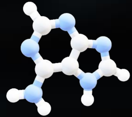
Nitrogen base
