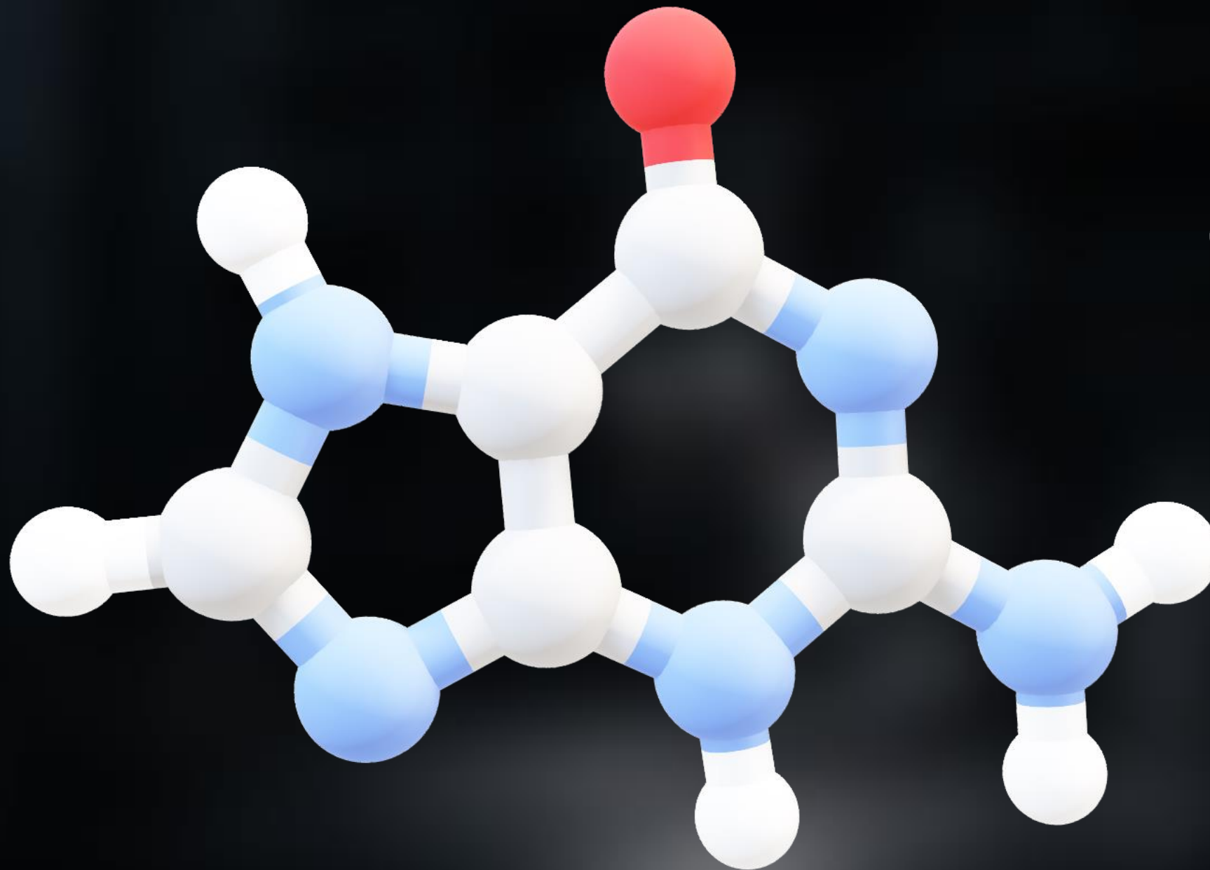
Guanine
